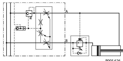
Fig. 5 Pressure controlled spool
