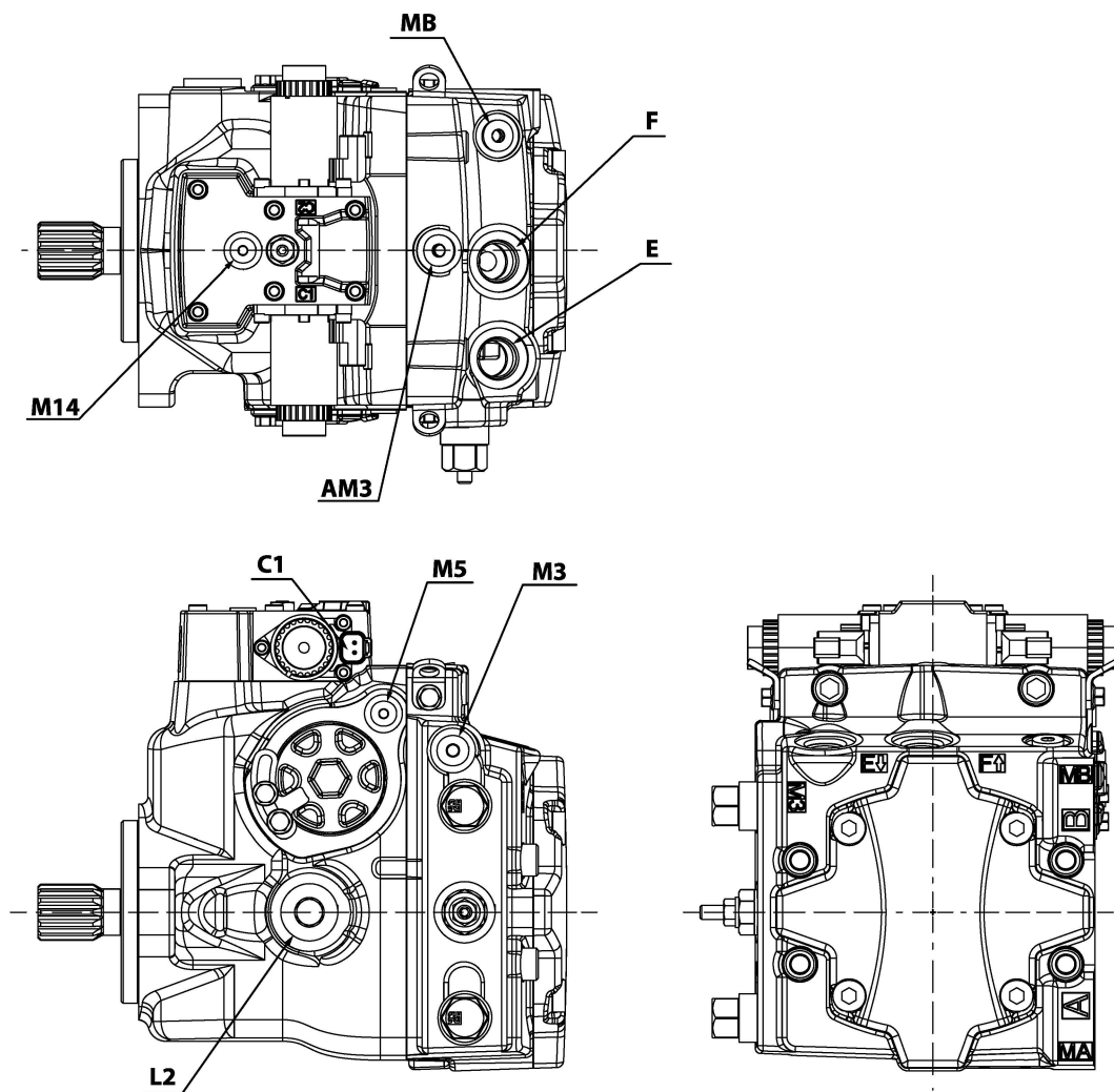
Ports description (ports per ISO 11 926-1)
