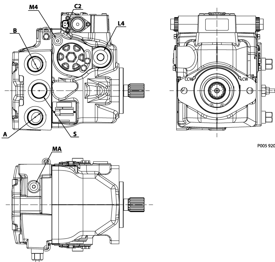
Ports description (ports per ISO 11 926-1)
