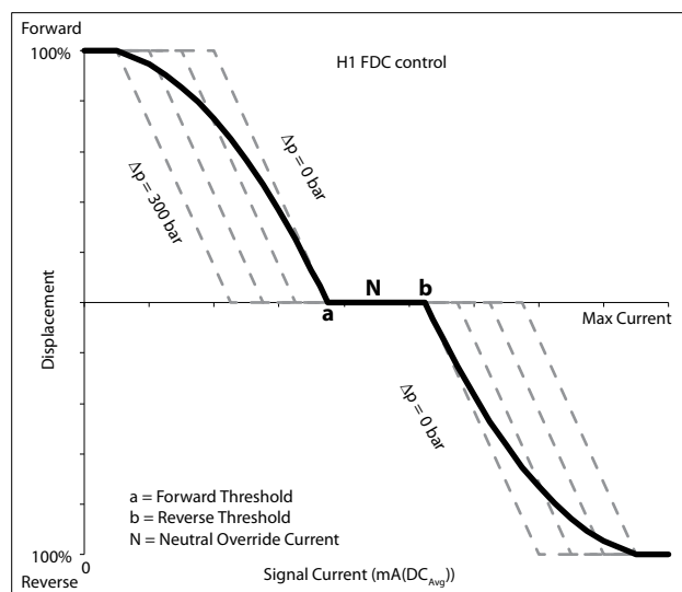
Pump displacement vs. control current
