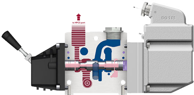
Maximum pressure for P- and T-port
