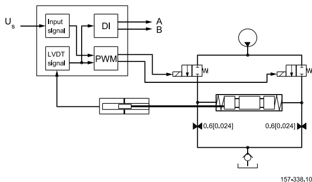
Hydraulic variant: PVEA
