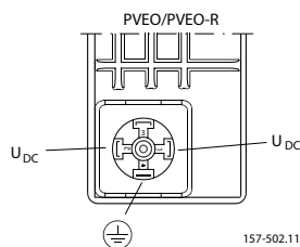
Hirschmann/DIN version of PVEO / PVEO-R
