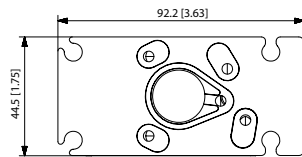
PVHC with Deutsch® connector
