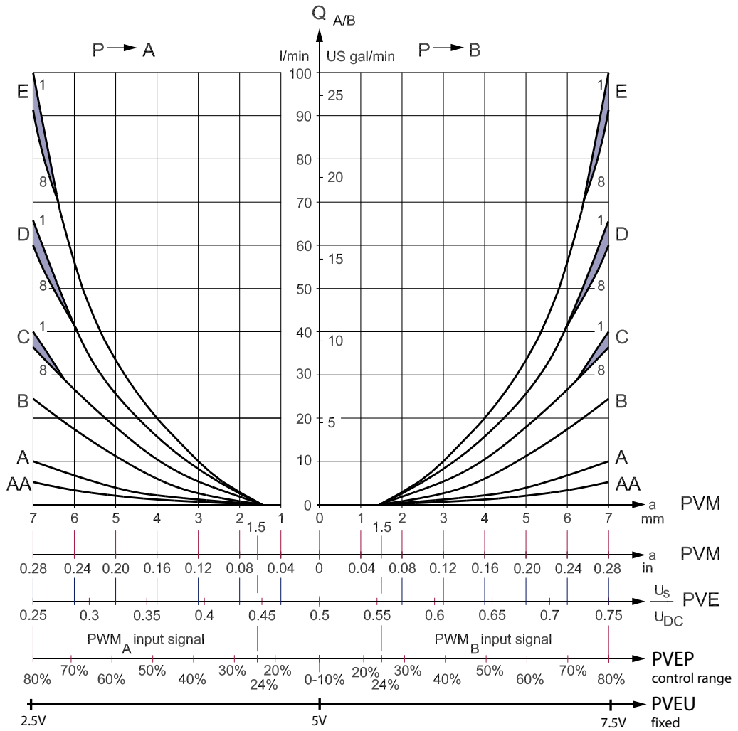
PVE characteristic – control by voltage
