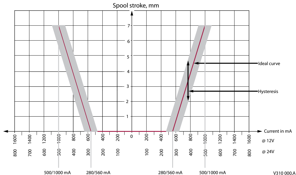
PVHC characteristic
