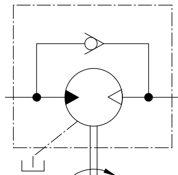
Valve schematic diagram
